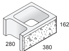
STANDARD CORNER UNIT
