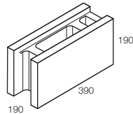
20.92 Double 'U' Corner 13.5kg 75 per pallet
