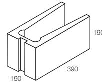
20.14 Deep Lintel Sash 15.2kg 110 per pallet
