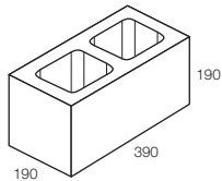
20.01 Standard Block/Double Corner 15.3kg 90 per pallet
