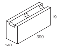
15.42 Recessed Web 11.0kg 95 per pallet
