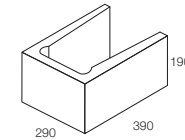
30.14 Full End 20.8kg 70 per pallet
