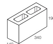
15.22 Special Corner 11.2kg 110 per pallet
