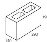
15.02 Three Quarters 10.7kg 140 per pallet
