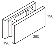
20.91 Double 'U' Block 15.3kg 75 per pallet
