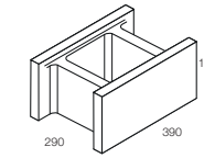
30.91 Double 'U' Block 21.7kg 55 per pallet
