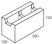
20.42 Recessed Web 15.9kg 90 per pallet
