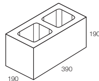
20.201SB Standard Block/Double Corner 13.6kg 90 per pallet
